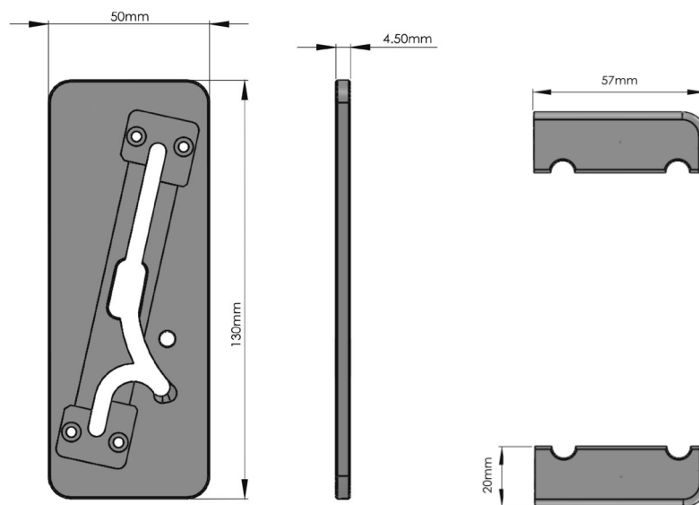
Ground plate
